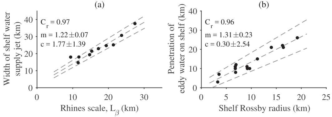
FIG. 10. Parameterizations for the cross-shelf extent from which the eddy can (a) extract water from and (b) push water onto the shelf. The dashed lines are regression lines of slope m and y-intercept c and their 95% confidence bounds. The C_r is the correlation coefficient.
