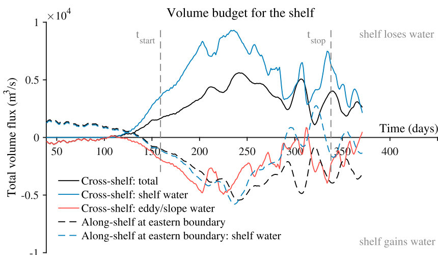
FIG. 5. Volume budget for the shelf, defined as a volume bounded by the two sponges, the coastal wall, and the shelf break. The export across the shelf break is compensated by an along-shelf jet moving water from the open eastern boundary into the shelf domain, as well as the onshore flow of eddy and slope waters.
