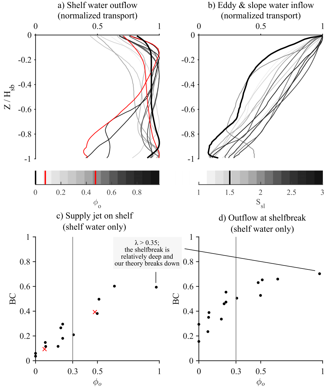
FIG. 9. (a),(b) Vertical profiles of the time-averaged shelf-water outflow and non-shelf-water inflow at the shelf break. The time average is over [t_{start}, t_{stop}] . The thick black lines are for a simulation with a flat shelf, \phi_o = 0 and S_{sl} = 1.5 . The inflow is always baroclinic while the outflow is only sometimes baroclinic (section 5). Values are normalized such that the maximum value in each profile is 1. (c),(d) The shelf-water supply jet is more baroclinic, as measured by BC in Eq. (9), for larger values of nondimensional parameter \phi_o (section 5b). Two simulations with \lambda = 0.22 are highlighted in red in (a) and with a red \times in (c). Despite the similarity in vertical structure of forcing, one profile is a lot more baroclinic than the other.
