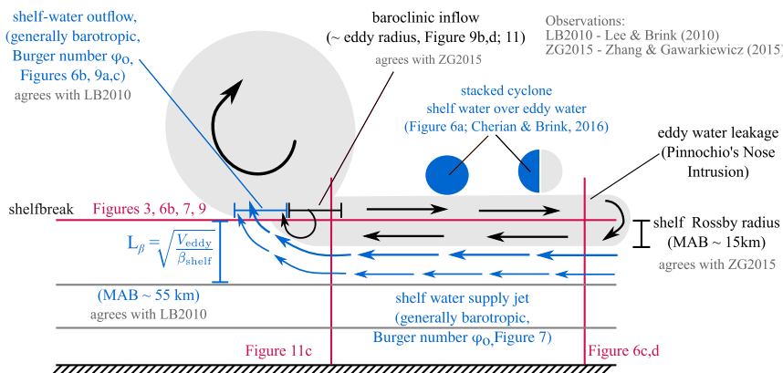
FIG. 4. Schematic flow field forced by a deep-water eddy at the shelf break.
